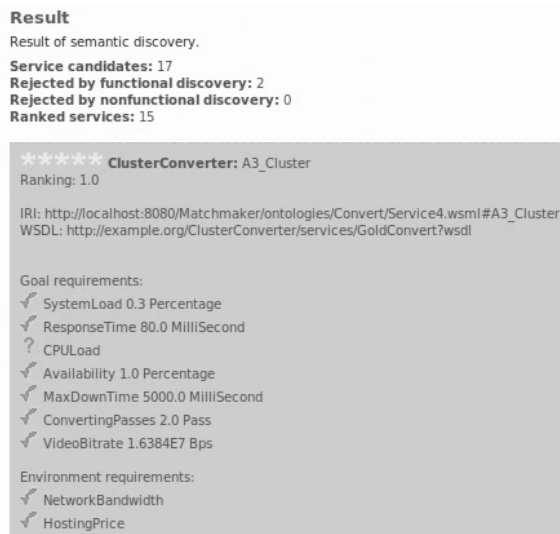
Figure 10: Screenshot of the weighted result listing following a query in the ConQo Cockpit discovery menu
