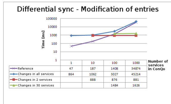
Figure 7: Scalability measured during a differential master-slave transfer of modified entries
