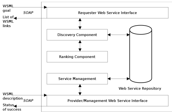
Figure 5: Architecture of the ConQo registry and discovery
