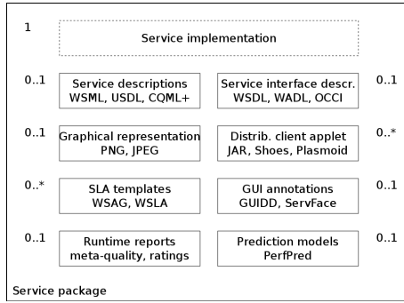
Figure 3: Service package according to the Tradeable Services Model
