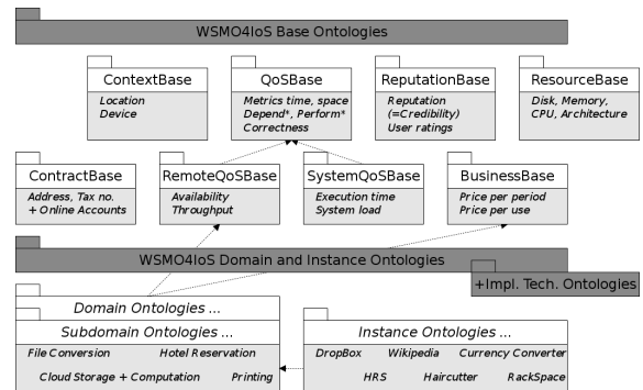
Figure 2: WSMO4IoS: Ontologies for the Internet of Services and Everything-as-a-Service
