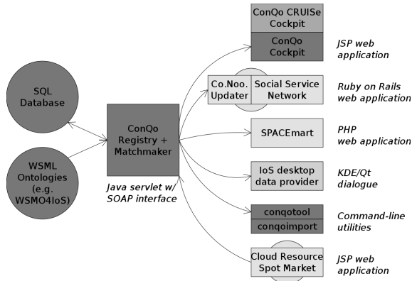
Figure 6: Usage and integration scenarios for the ConQo service registry
