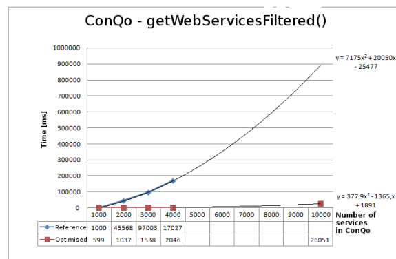
Figure 8: Increased scalability after combined refactoring and code improvements
