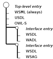
Figure 4: Structure of entries in the registry
