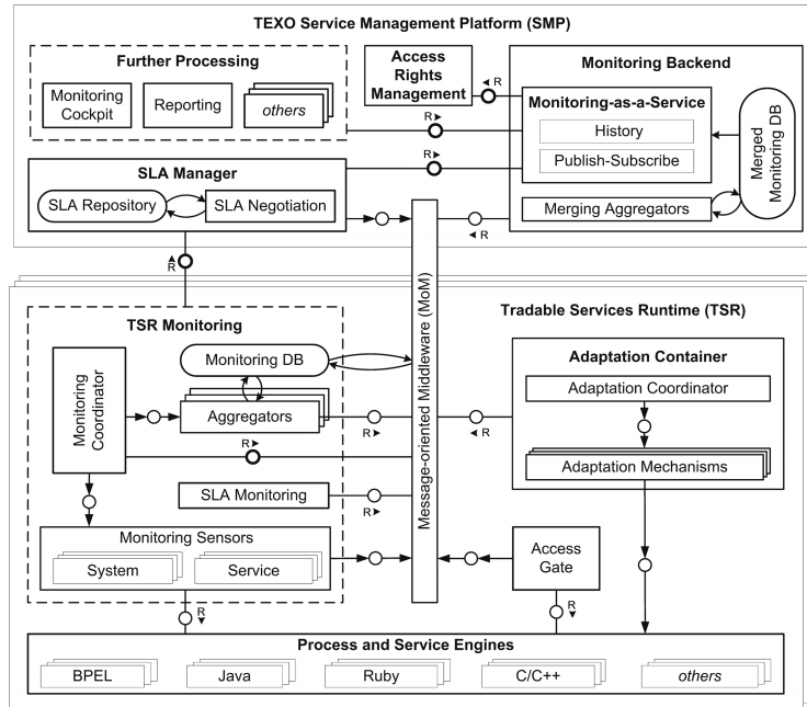
Fig. 4. Contracting and monitoring architecture for the IoS
